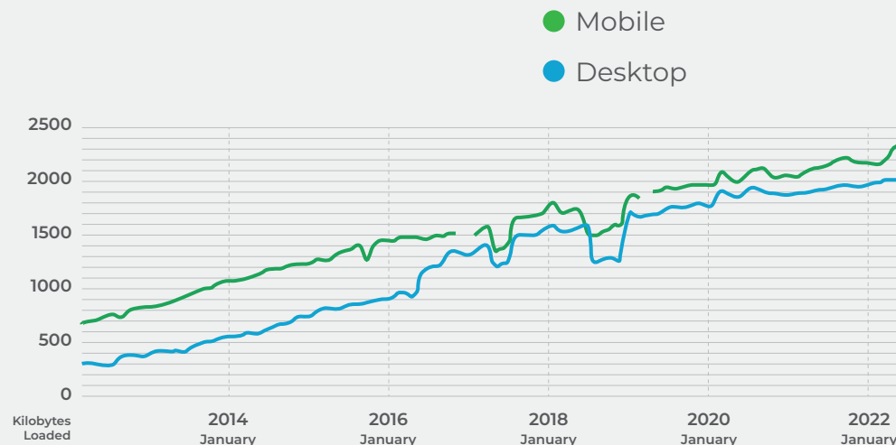
Median Page Weight Over Time
