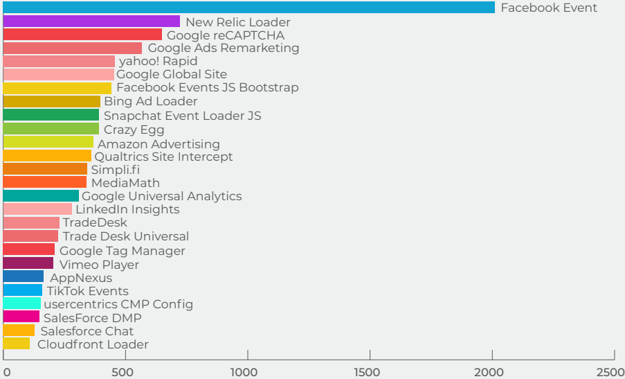
Most Common Duplicate Tags
